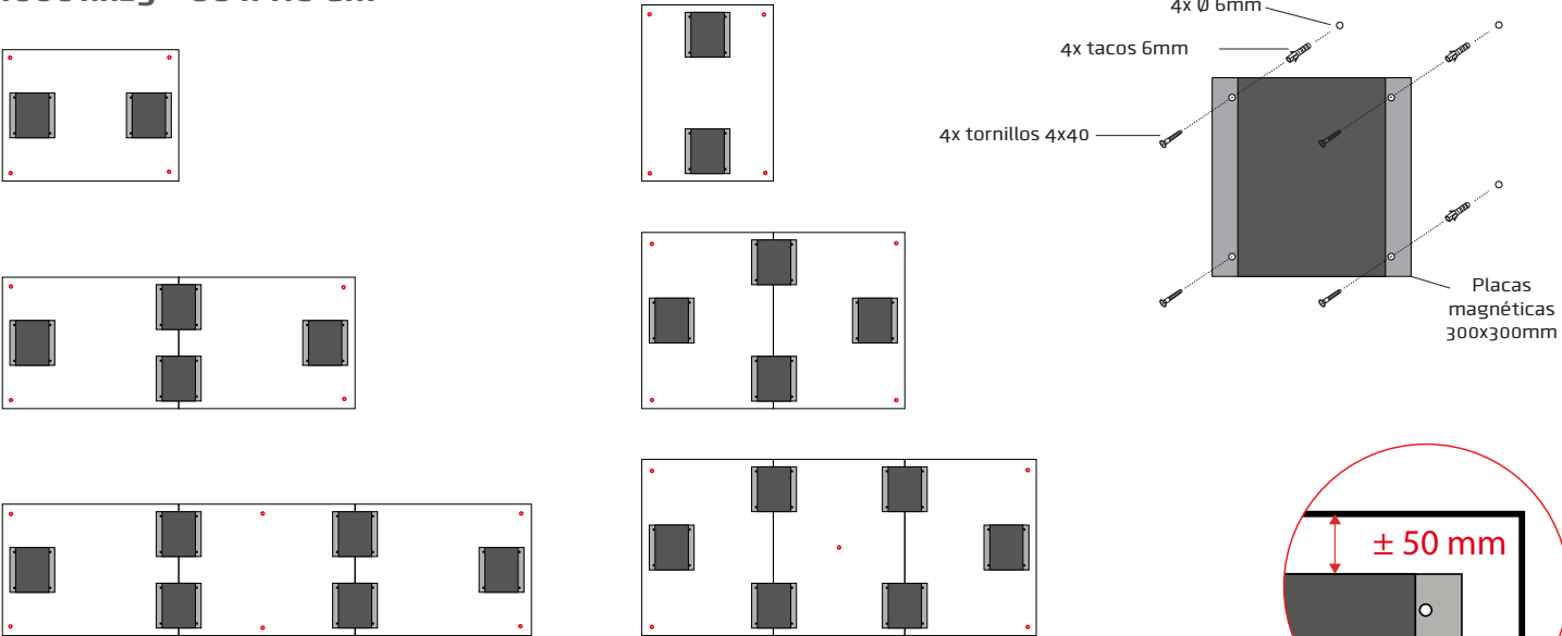
16001.x29 - 88 x 118 cm
